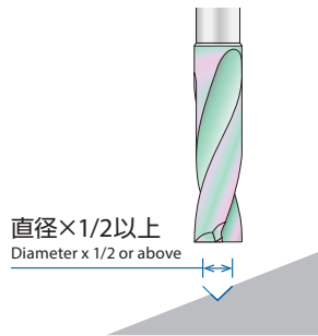
傾斜部加工 Machining an inclined plane
