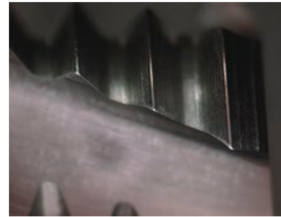
2本目 8,800穴加工後 No.2 (after cutting 8,800 threads)
